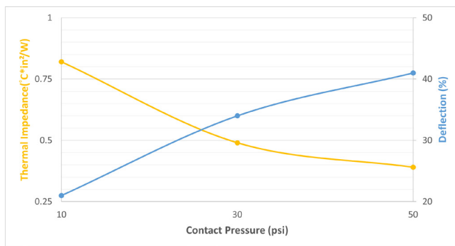
Contact Pressure, Thermal Impedance, and Deflection
