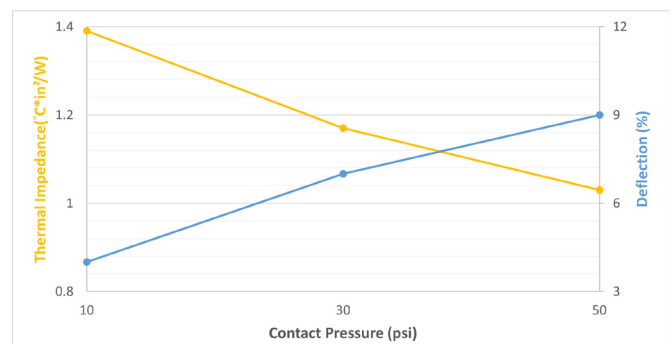
壓力, 熱阻抗, 變形量示意圖 Contact Pressure, Thermal Impedance, and Deflection
