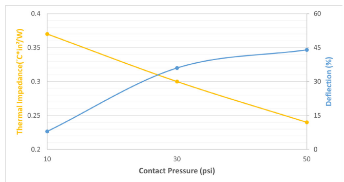
压力, 热阻抗, 变形量示意图 Contact Pressure, Thermal Impedance, and Deflection
